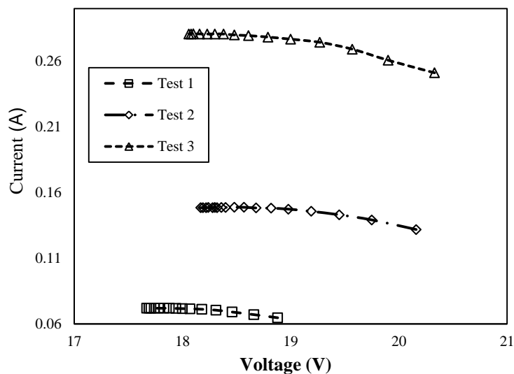
148 Figure 2: Variations of current as function of voltage under different radiation
